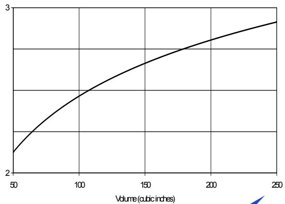
Primary to Bubble Ratio (Out-128 Hz)
